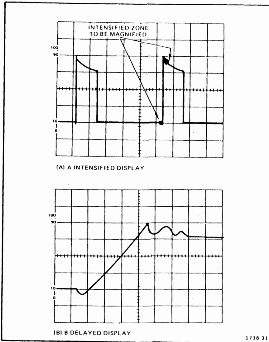
Fig. 24. Delayed sweep magnification.
