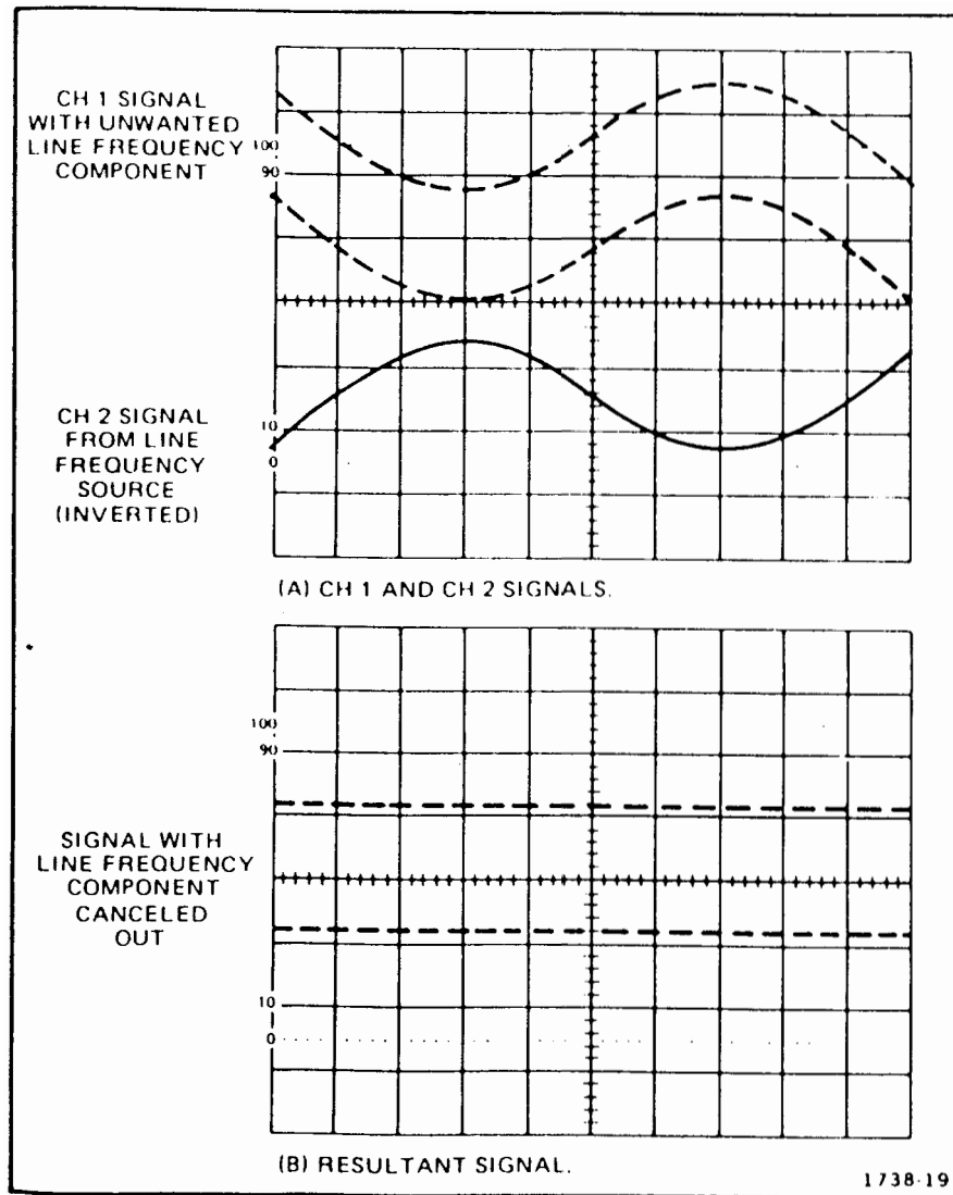
Fig. 17. Common-mode rejection.
