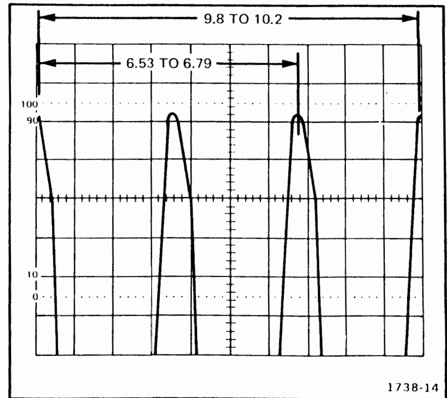
Fig. 12. Basic 475A timing check.
