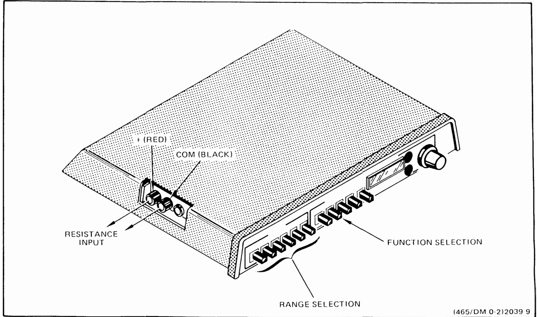
Fig. 8. Resistance.
