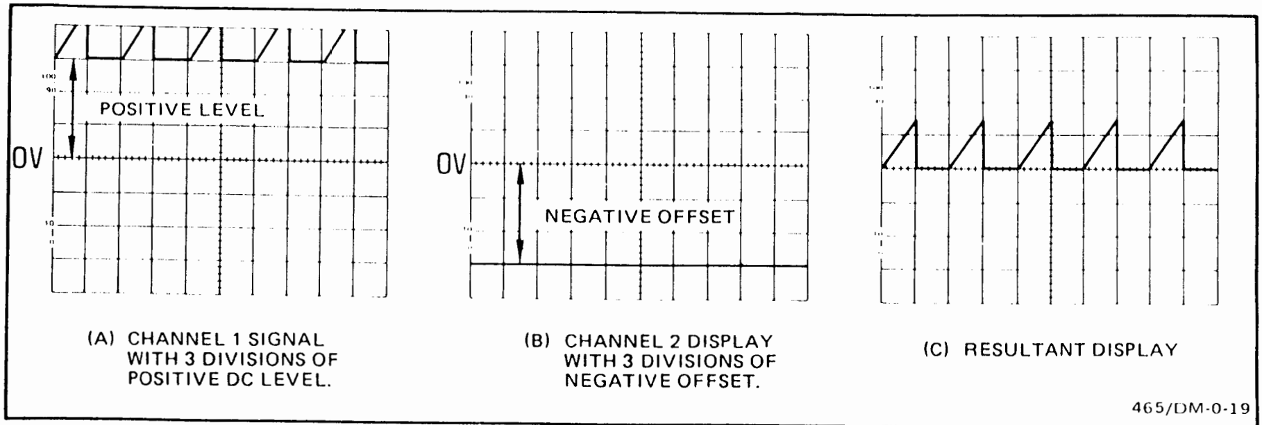
Fig. 16. Algebraic addition.
