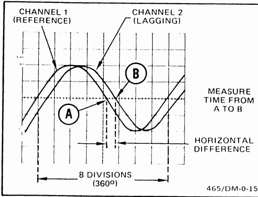
Fig. 21. Phase difference.
