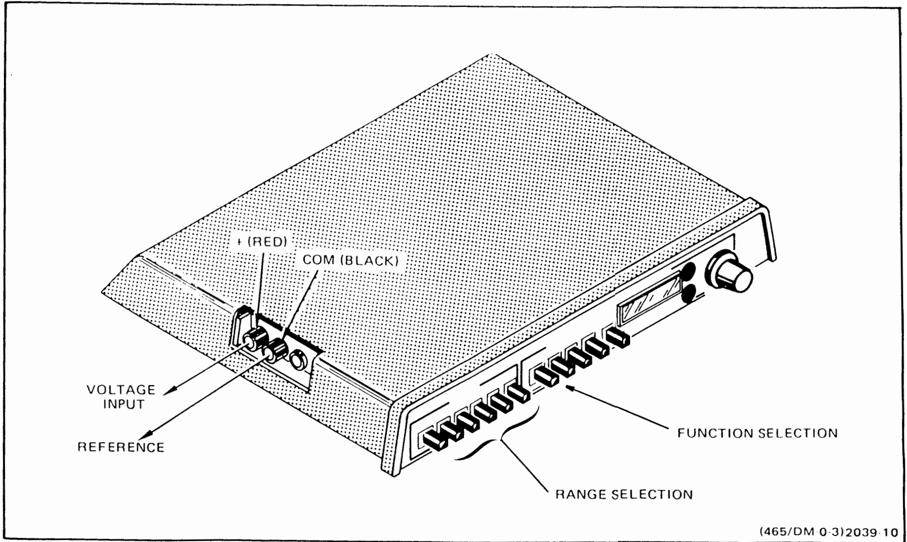
Fig. 9. Volts.
