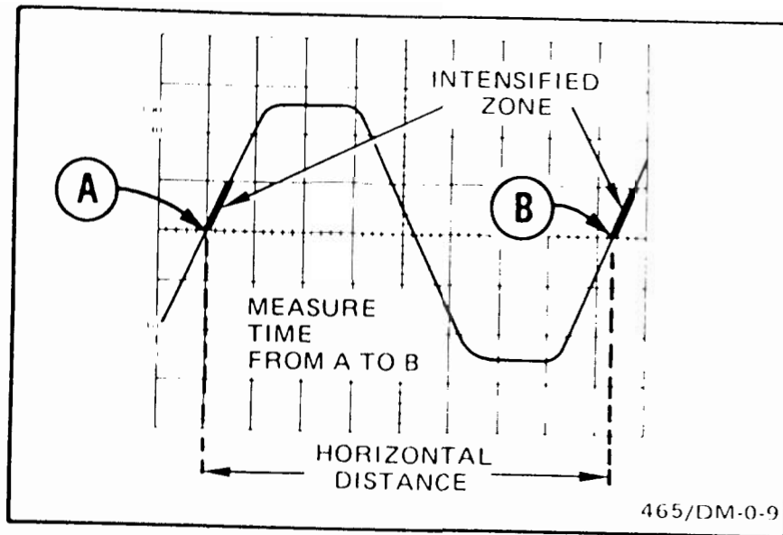
Fig. 26. Time duration.
