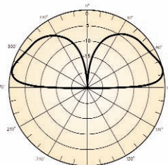
Typical elevation radiation pattern
